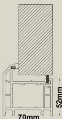
Standard PVCu
