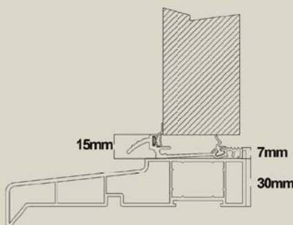
Mobility threshold on a PVCu Cill
